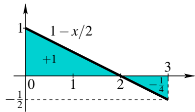
FIGURE VI.2 – \int_{[0,3]} 1 - \frac{1}{2}x dx
