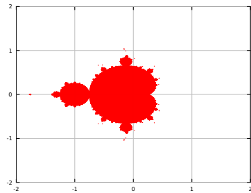
FIGURE II.13 – Ensemble de Mandelbrot
