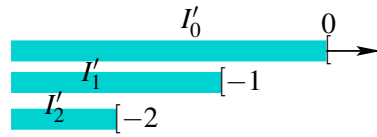
FIGURE IV.3 — \bigcap_{n \in \mathbb{N}} I'_n = \emptyset
