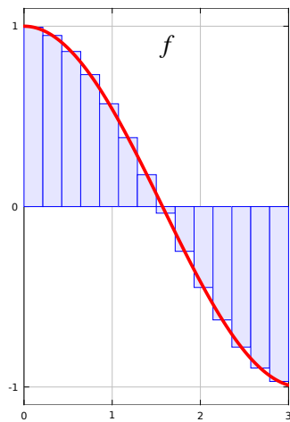
FIGURE VI.4 — I_{x_0, \dots, x_n}(f)
