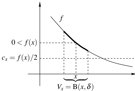
FIGURE IV.4 — f \geq c_x localement
