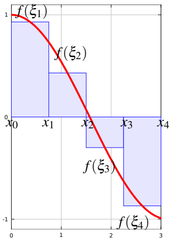
FIGURE VI.3 — I_{x_0, \dots, x_n}(f)
