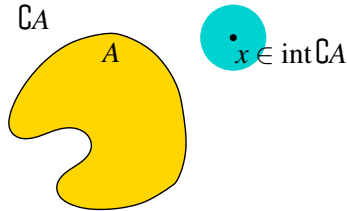
FIGURE III.5 – \complement \text{adh}A = \text{int} \complement A
