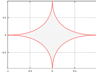
FIGURE II.8 – B_{|\cdot|_p}[0, 1] pour p < 1
